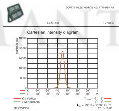
OFCC1_DCP776 1xLED-HBRGB +ZCP770 BSP A8.EPS
