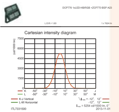
OFCC1_DCP776 1xLED-HBRGB +ZCP770 BSP A23.EPS
