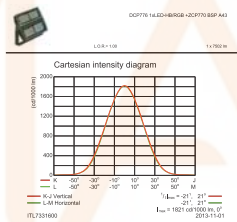
OFCC1_DCP776 1xLED-HBRGB +ZCP770 BSP A43.EPS
