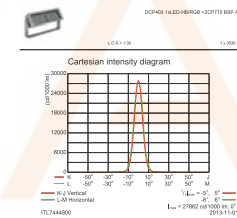
OFCC1_DCP403 1xLED-HBRGB +ZCP770 BSP A8.EPS
