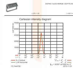
OFCC1_DCP403 1xLED-HBRGB +ZCP770 A5.EPS
