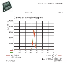
OFCC1_DCP776 1xLED-HBRGB +ZCP770 A5.EPS
