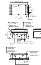
Power/data supply units ZCX400
