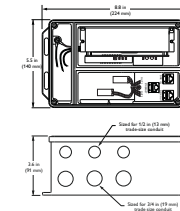
Power/data supply units ZCX400
