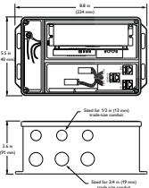
Power/data supply units ZCX400
