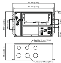
Power/data supply units ZCX400
