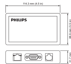
Power/data supply units ZCX400
