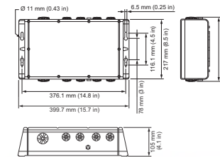
Power/data supply units ZCX400
